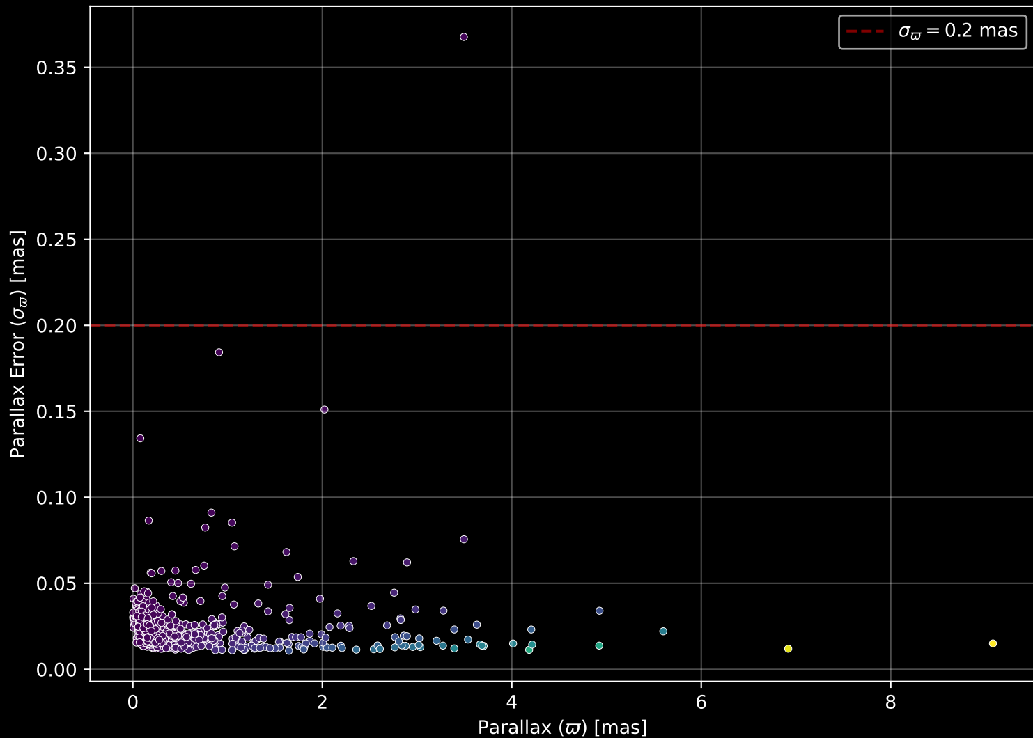
APOGEE DR17 Field: [M71] Parallax Quality (n= 833)
