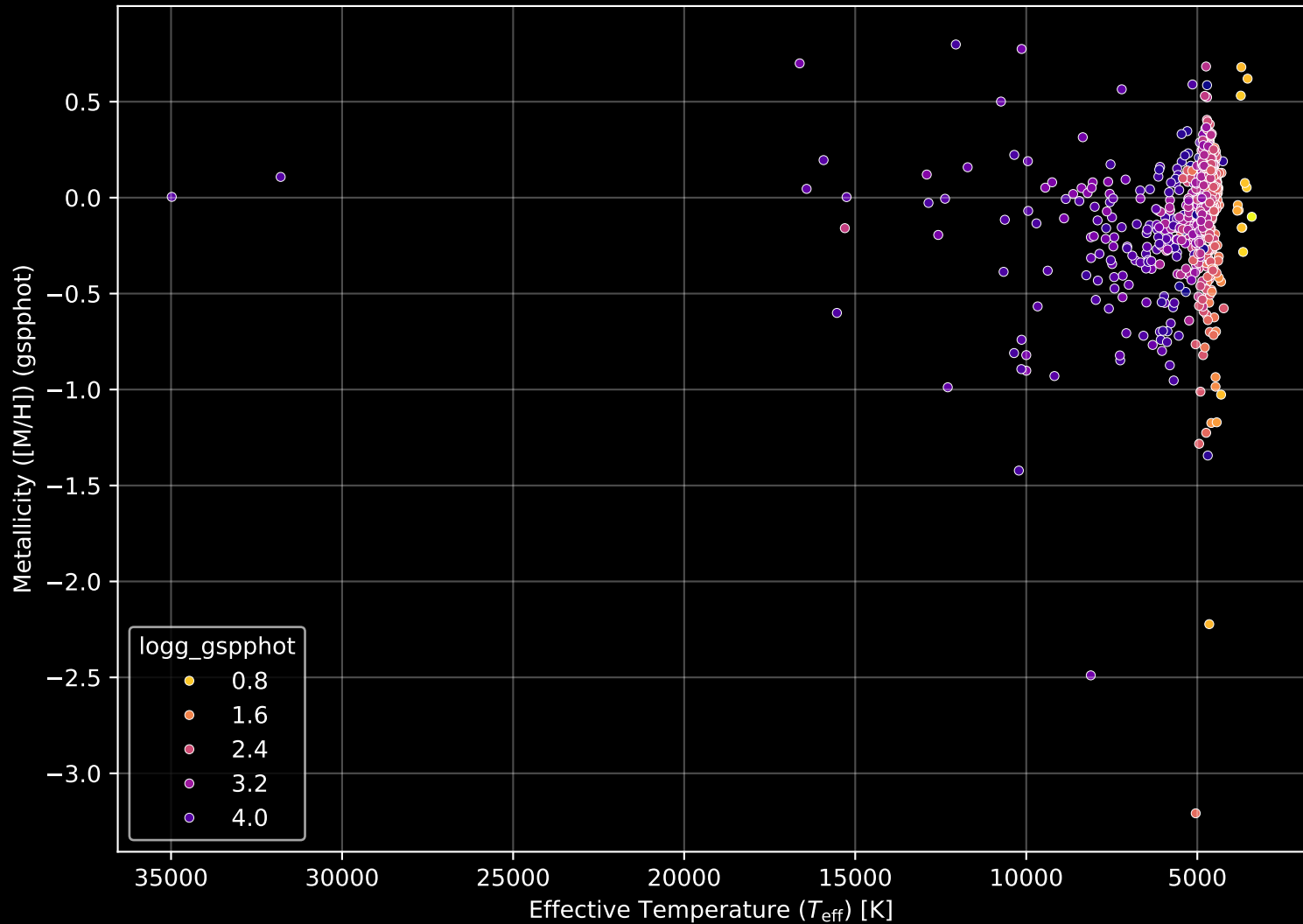
APOGEE DR17 Field: [M71] Stellar Population Parameters (n= 833)
