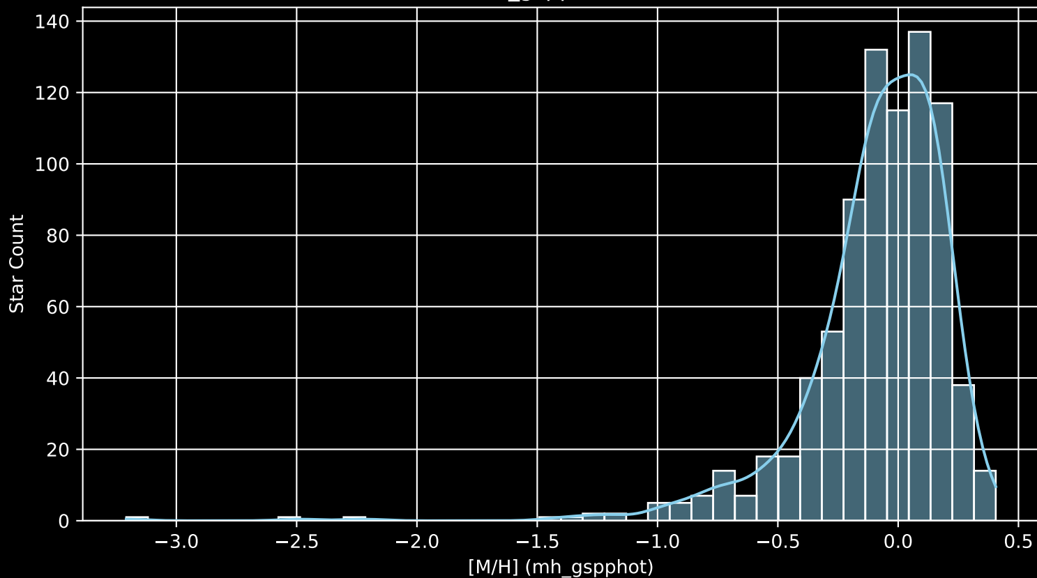
APOGEE DR17 Field: [M71 [M/H] (mh_gspphot) (n= 819)
