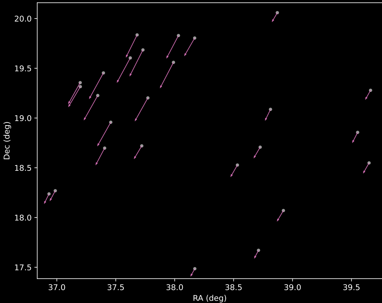
APOGEE DR17 Cluster 32 Proper Motion Vectors (n=26)
