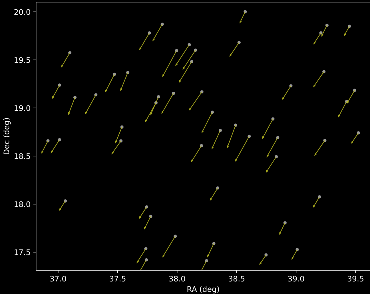
APOGEE DR17 Cluster 36 Proper Motion Vectors (n=52)
