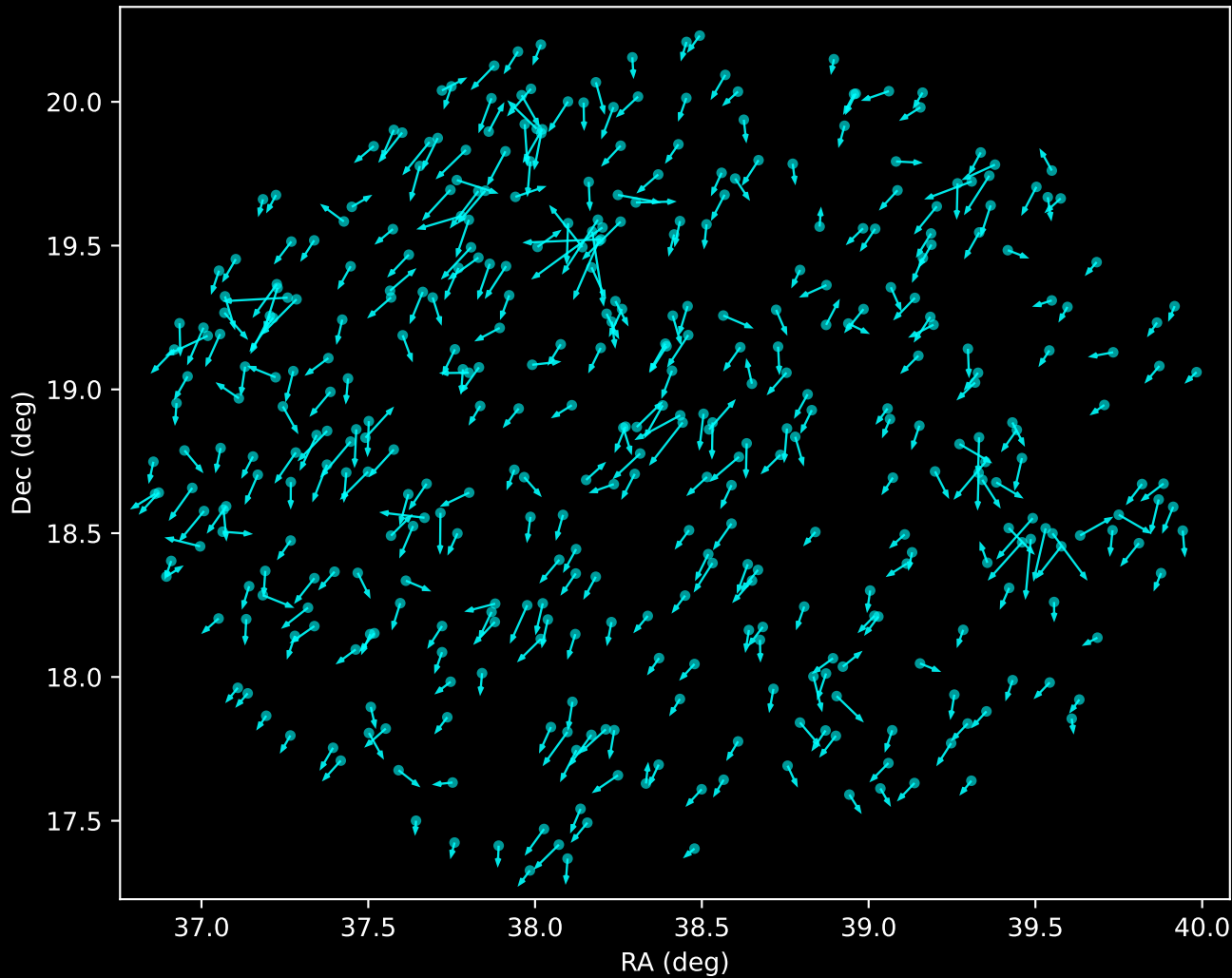
APOGEE DR17 Noise Stream Proper Motion Vectors (n=403)
