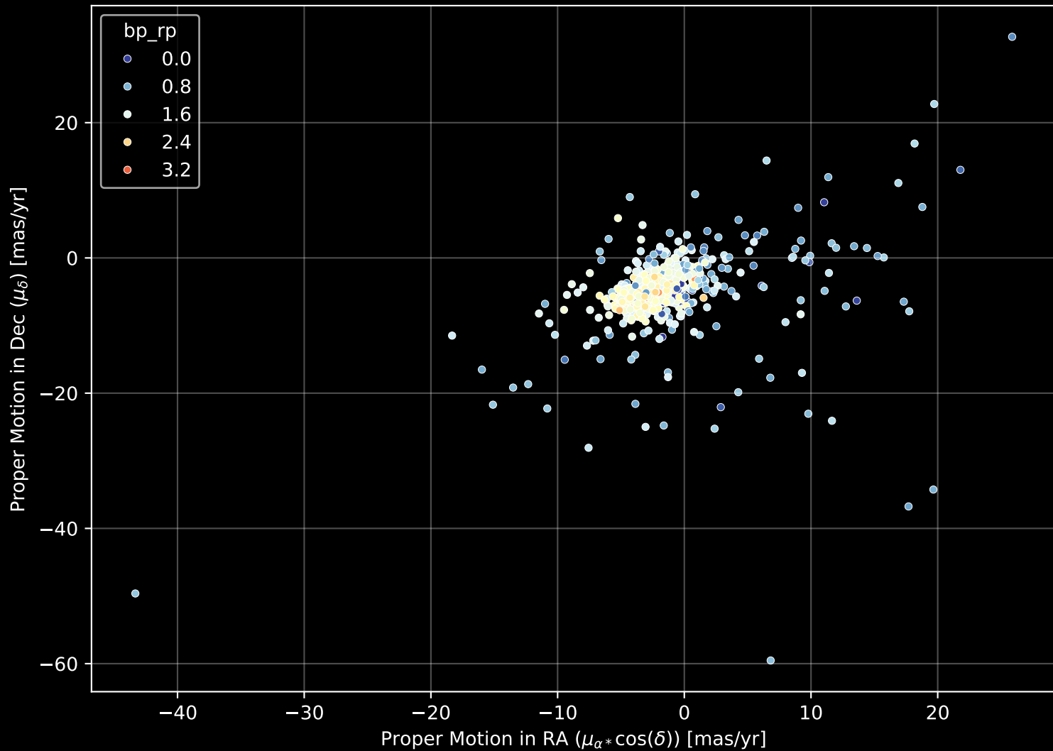
APOGEE DR17 Field: [M71] Proper Motion Diagram (n= 833)
