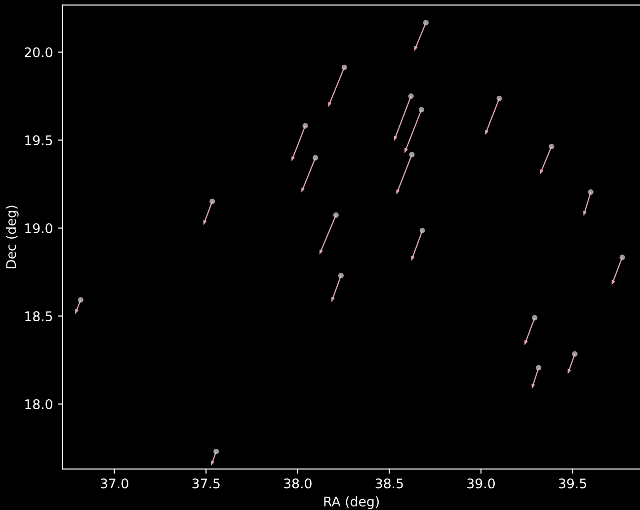
APOGEE DR17 Cluster 33 Proper Motion Vectors (n=20)
