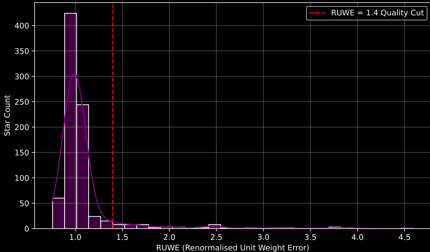
GAPOGEE DR17 Field [M71] RUWE Distribution (n= 827)
