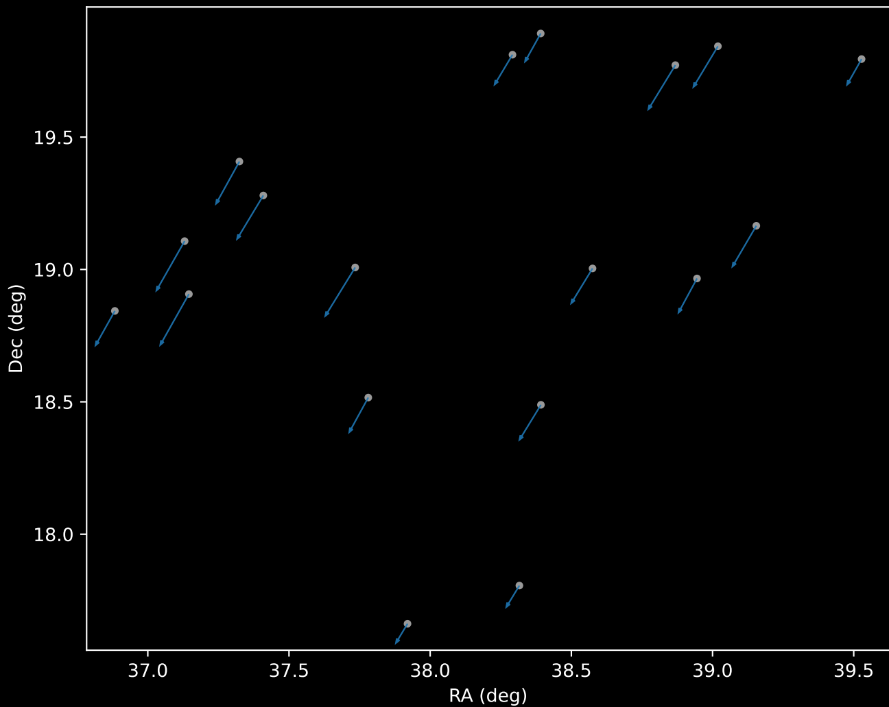
APOGEE DR17 Cluster 40 Proper Motion Vectors (n=18)
