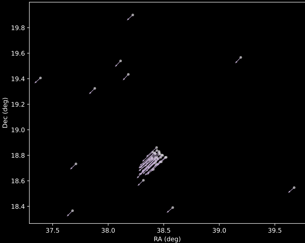
APOGEE DR17 Cluster 9 Proper Motion Vectors (n=37)
