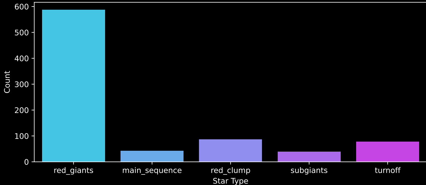
APOGEE DR17 Field: [M71] Count plot of Star Type
